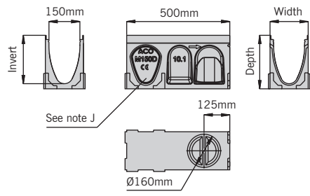
M150D 0.5m constant depth channel
