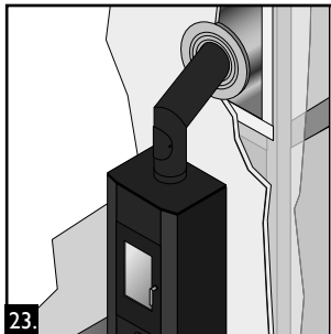
23. Finished installation.
