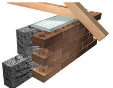
Cavity Closers
